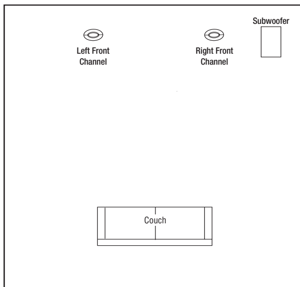
Figure 1. In this overhead view of a typical installation, satellite speakers are used to reproduce sound for the front channels. The powered subwoofer provides bass for effects and music.
