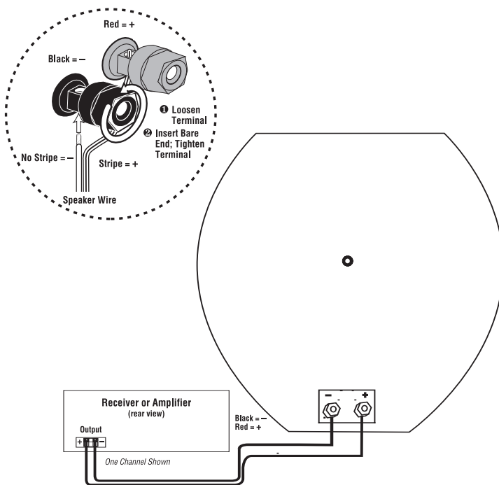
Figure 3. Wiring diagram shows polarity connections for one channel of a home theater system.
